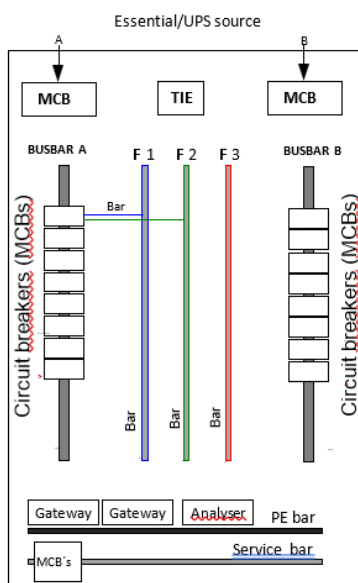
Figure 1: typical internal QCC panel arrangement
