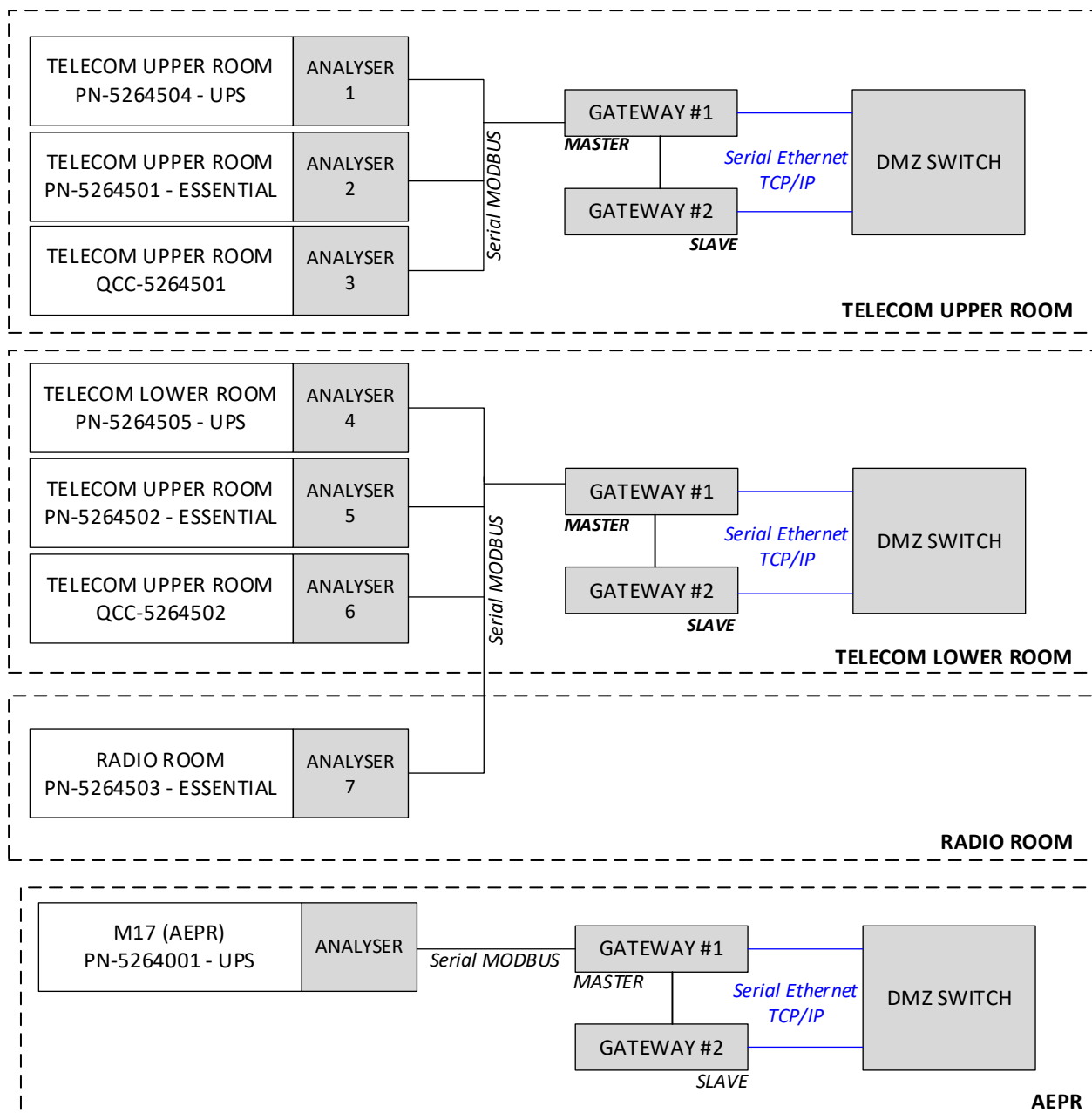
Figure 5: schematic interconnections
