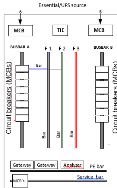
Figure 2: typical internal AC panel arrangement
